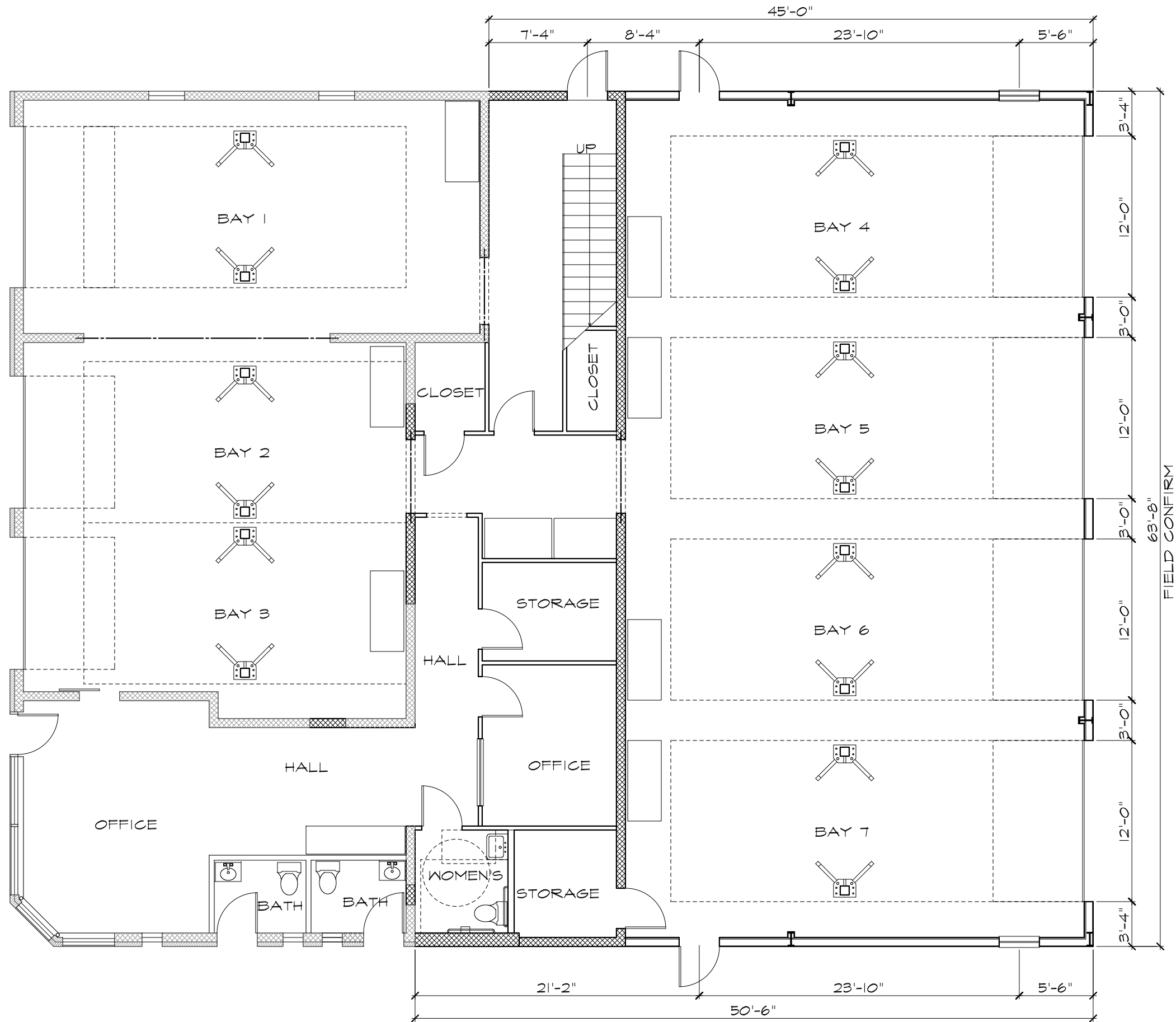
1 FIRST FLOOR PLAN - SCOTT'S IVY EXXON
